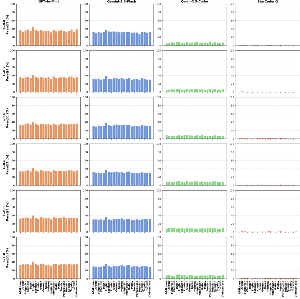
Fig. 9 pass@1 for C++ across 23 non-English prompt languages, grouped by language family.
