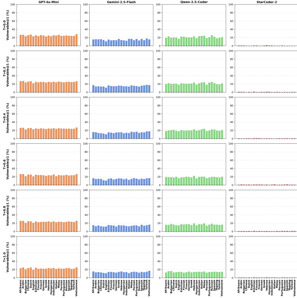
Fig. 16 Vulnerable@1 across CWEs per model and temperature for Java.
