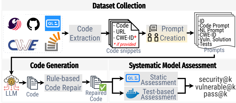
Fig. 2 Framework overview
